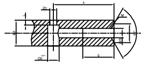
A-DETAYI (D8-D14)
