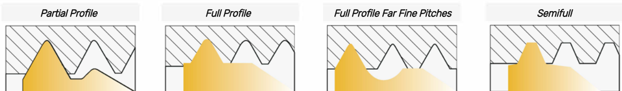
The V partial profile insert cuts without topping the outer diameter of the thread. The same insert can be used for a range of different thread pitches which have a common thread angle.
