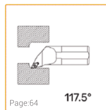
S...TWLNR/L
