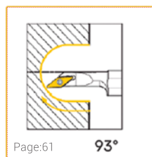
S...TDQNR/L
